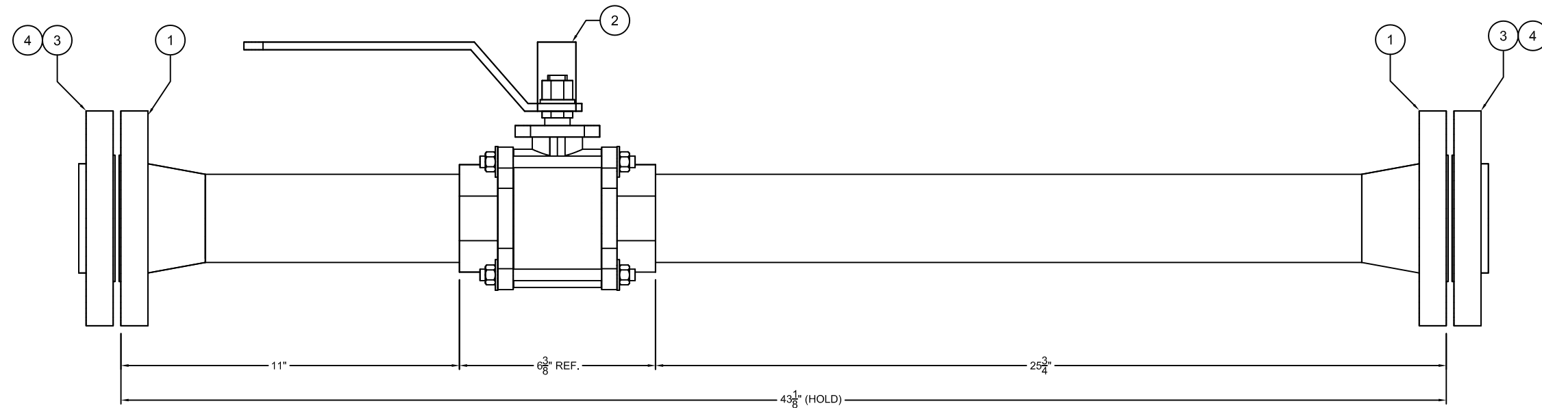
FUEL SPOOL FRONT VIEW SCALE: 3"=1'-0"
