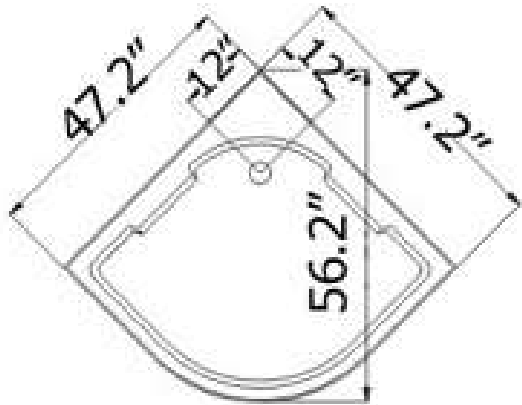
Drawing for DZ962 Specification: 47.2" x 47.2" x 89"
