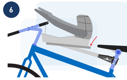
Step Six Position the seat on the arm as far forward as possible without interfering with your handle bars or steering post.
