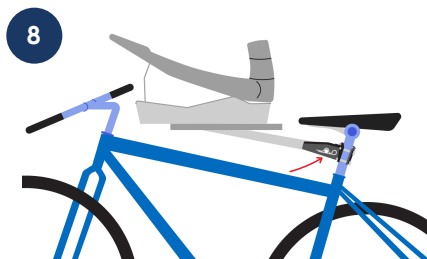
Step Eight Install the assembled pet seat to the bicycle using the quick release pin and be sure to secure that with the cotter pin provided or a small pad lock.
