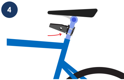
Step Four Attach the receiver to your bicycle seat post. There must be at least 1.75 inches of post exposed below the seat to make this connection.
