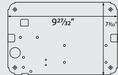
MOUNTING VIEW
