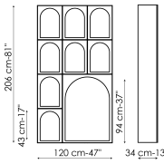
Combination 3 Width: 120cm Depth: 34cm Height: 206cm
