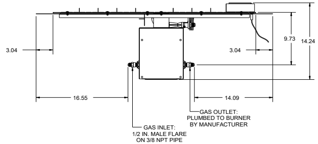
BURNER FRONT ELEVATION
