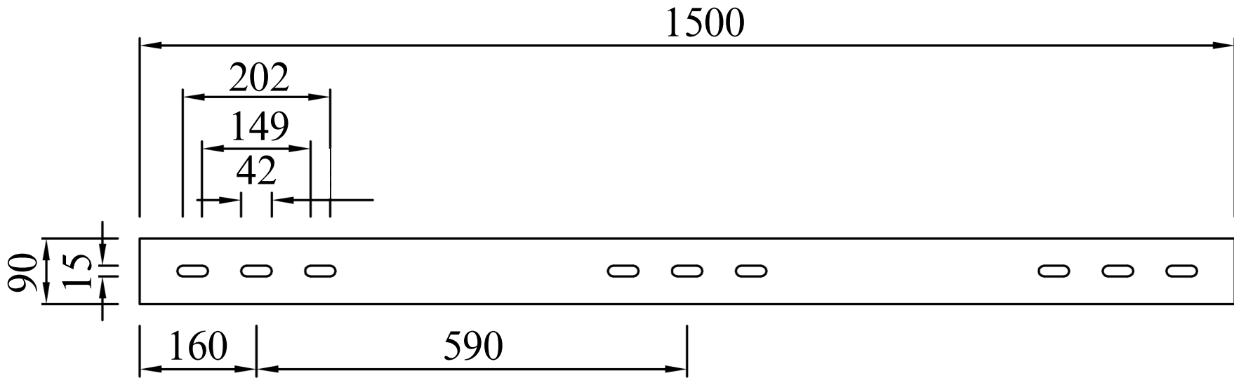
Plan View
