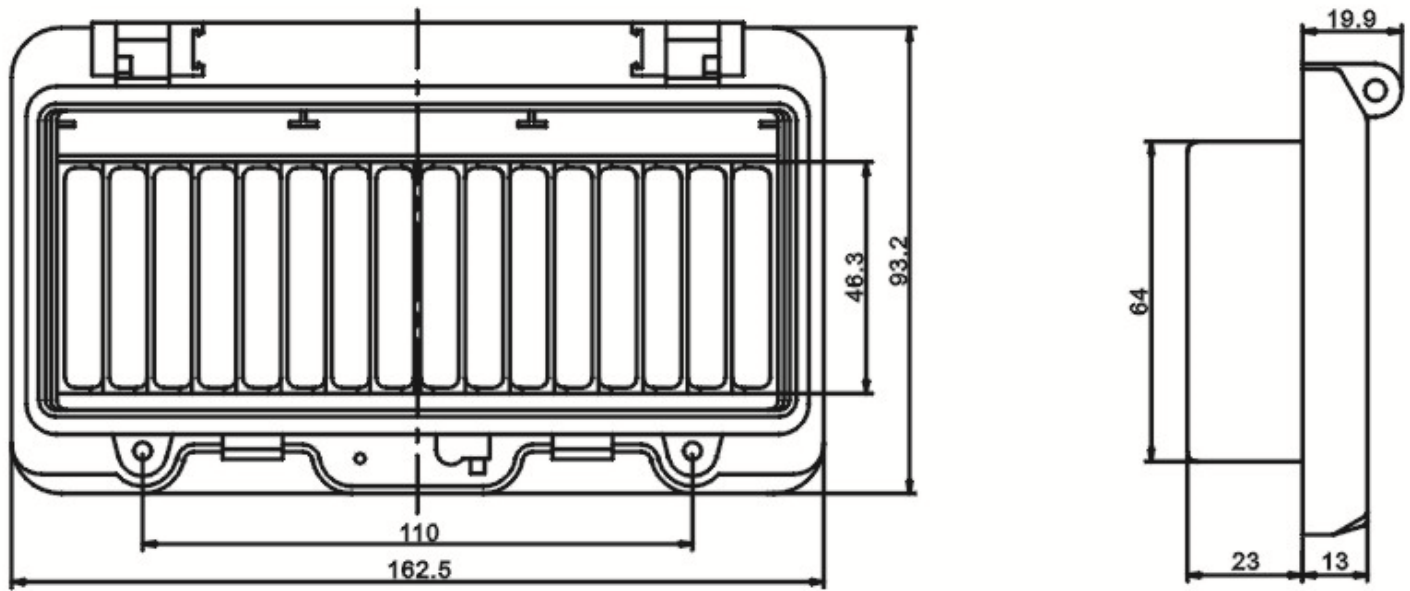
Rear protective box external dimensions (mm)
