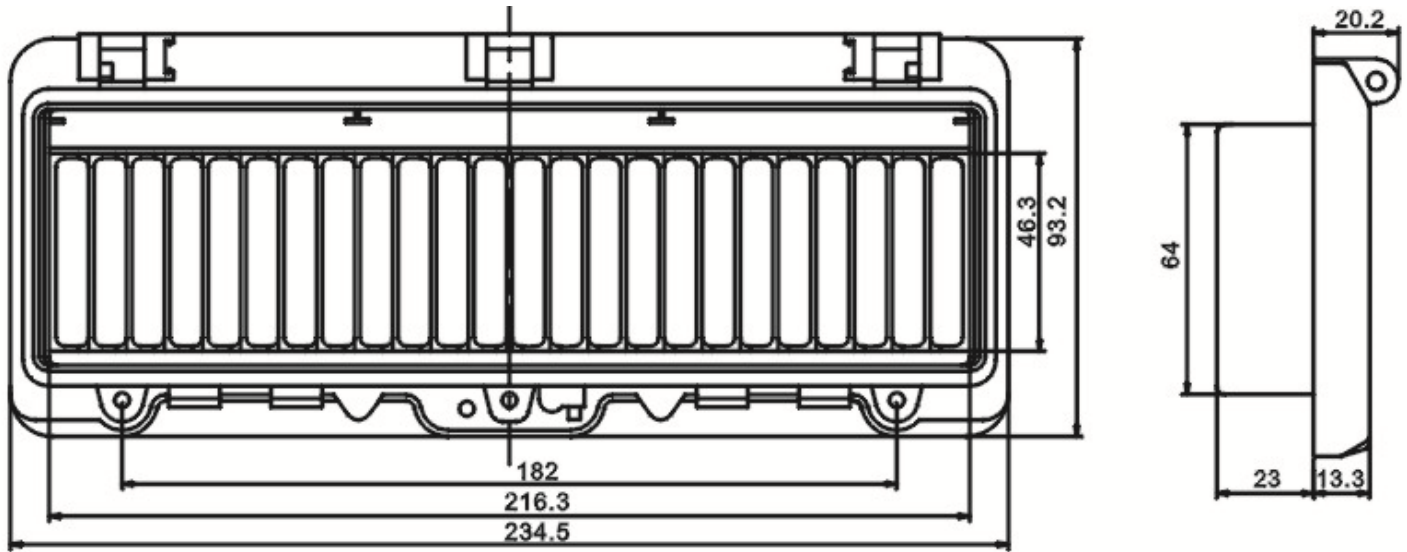
Rear protective box external dimensions (mm)
