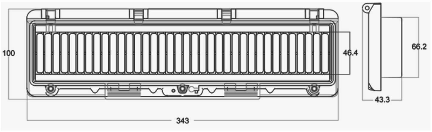
Rear protective box external dimensions (mm)
