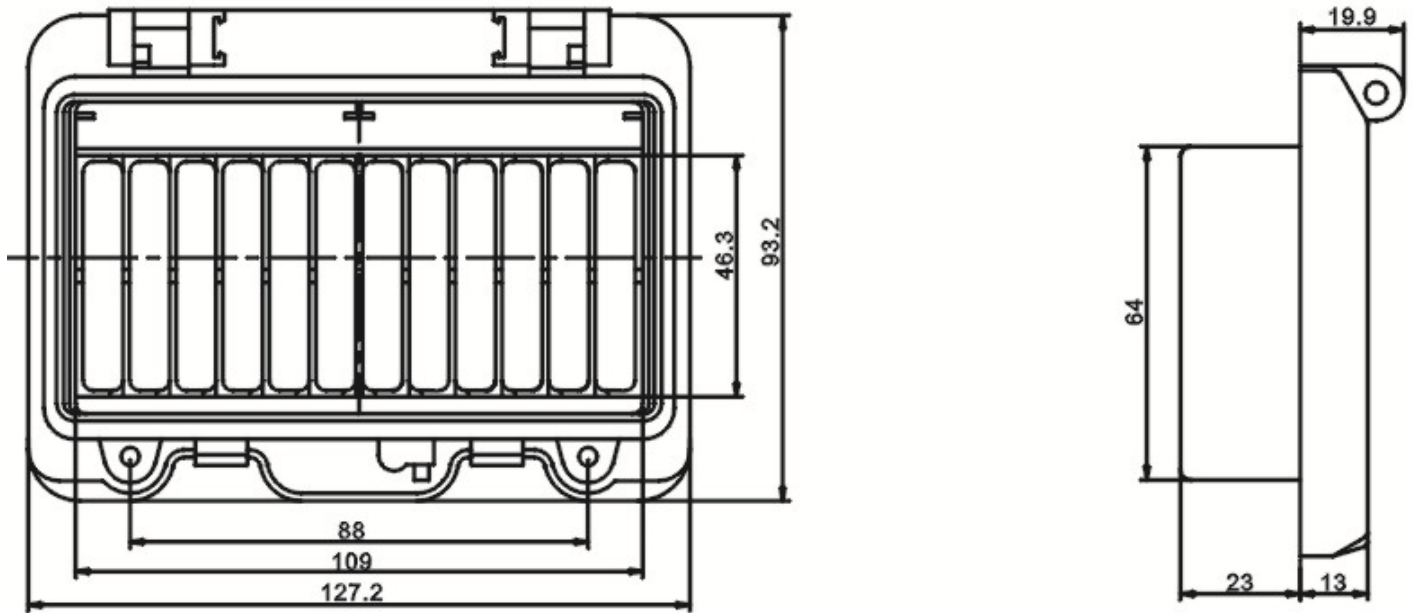
Rear protective box external dimensions (mm)
