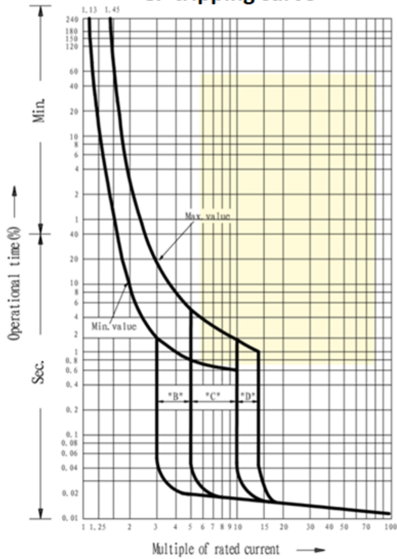
CP tripping curve
