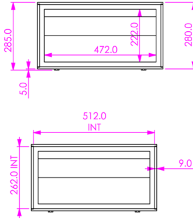
FRONTAL VIEW
