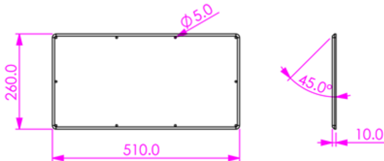
END PLATE
