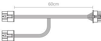
F PCIe 6+2 pin (2 connectors) x 3
