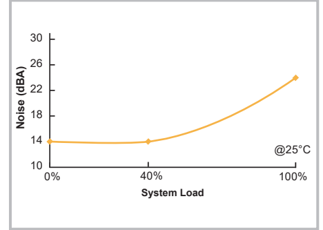
SAC (Smart Airflow Control) Design
