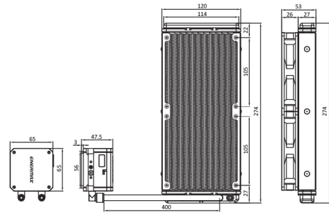
ELC-LMT240-W-ARGB
