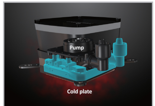
Dual Chamber water block design (patented)
