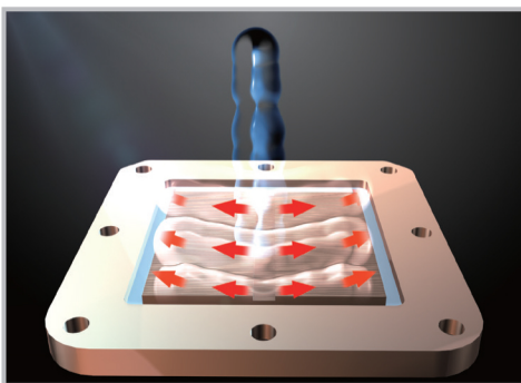
Central Coolant Inlet (CCI) design combined with patented Shunt-Chanel Technology (SCT) cold plate
