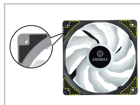
Anti-vibration rubber pads
