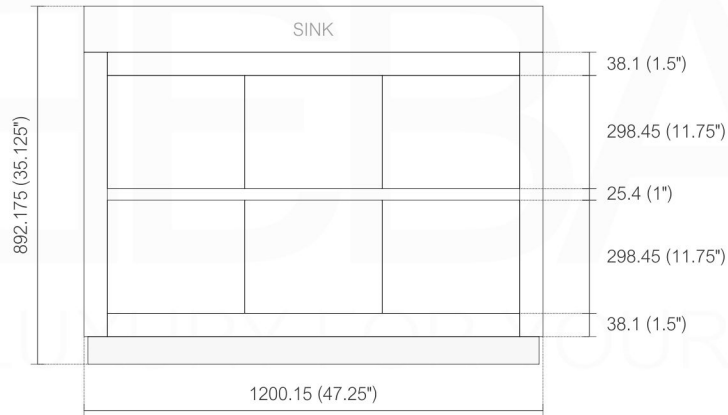
BACK ELEVATION
