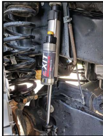
FRONT SHOCK 2018 FORD F350
