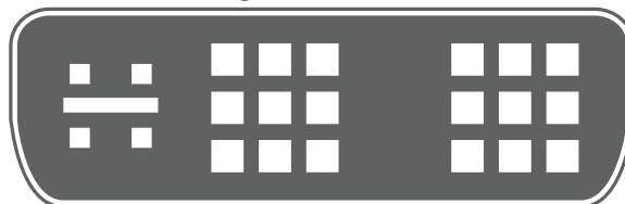
DVI-I Single Link
