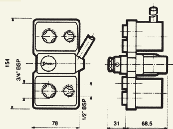
MM109.12/21-16 call for pricing 109.12mm mobile plate with 1/2", 3/4" inlet and outer female threaded collector.
