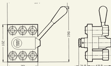
MM109.06DG17 call for pricing 109.06 mm mobile plate with 6 unit BSP 3/8" female threaded shut-off coupler (3 circuit).
