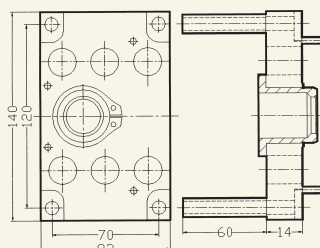
MK109.06 call for pricing 109.06 mk mould plate for 6 unit plugs (3 circuit)
