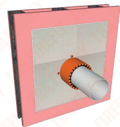
40-150mm OD uPVC Pipe through 120 Min FRL Fire Rated Plasterboard Wall Intubatt Seal
