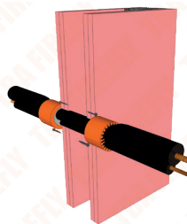
Nitrile Rubber Lagged Pair Coil through 120 Min FRL Fire Rated Plasterboard Wall
