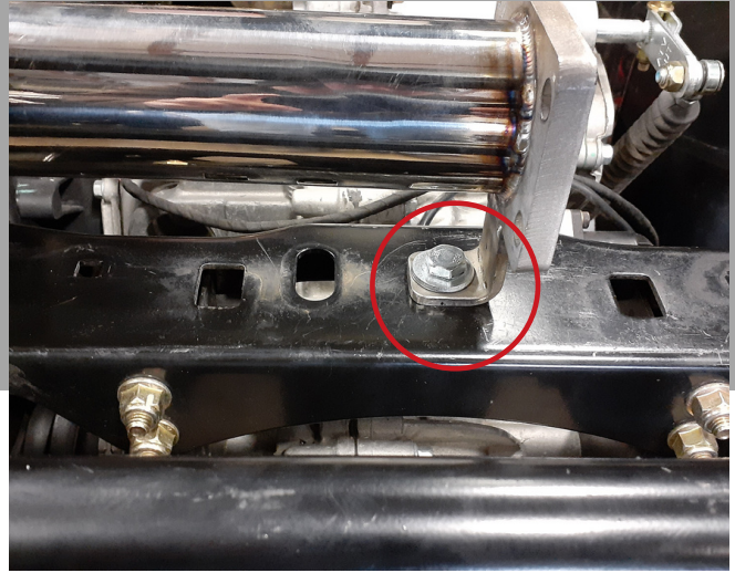
8. Set turbo assembly into chassis. Bolt down turbo assembly into vehicle. Tighten exhaust clamp and reinstall exhaust heat shielding. Reinstall stock O2 sensor and plug in
