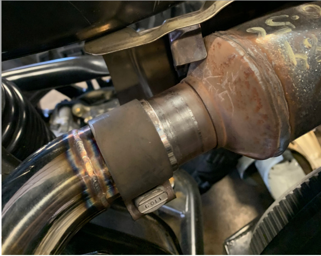
7. Install exhaust clamp onto turbo inlet pipe
