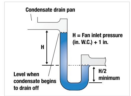
Figure 1c: Condensate Draining
