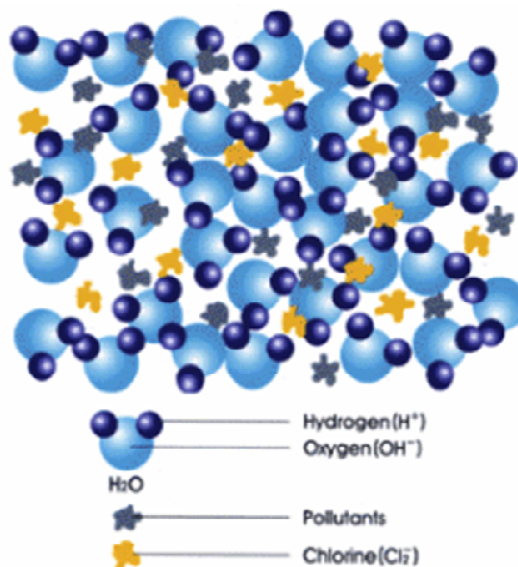
Unstructured Molecules
