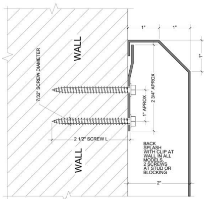
BACK SPLASH WALL ANCHOR WITH SS CLIP CL - DETAIL
