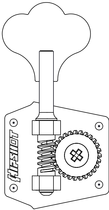
HB3 11/16" [17.5mm] HEADSTOCK HOLE
