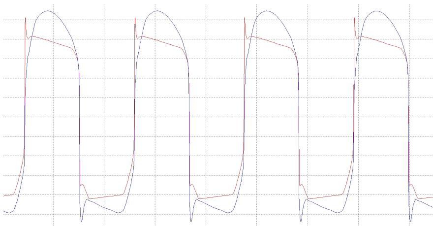
Figure 7. Response of the PAE-1 to a resistive load (red) and to a speaker load at its resonant frequency (blue).
