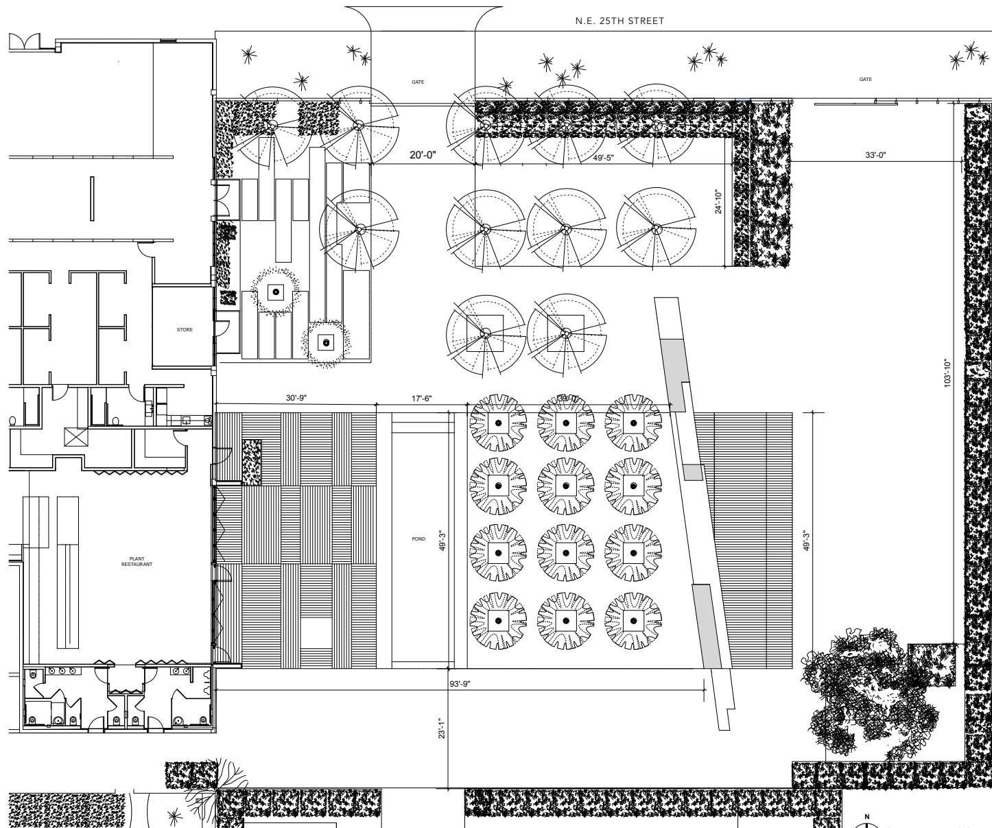
N GARDEN FLOOR PLAN A-1 scale: 1/16"=1'-0" 1
