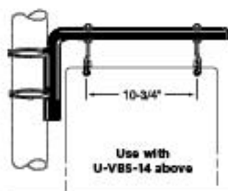
U-VBS-1 22" Vertical Bracket $20.00
