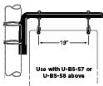
U-BS-1 28" Horizontal Bracket $29.95
