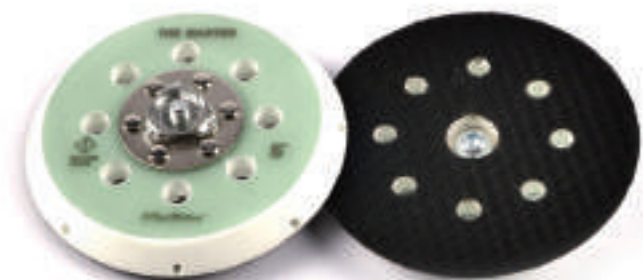
3011125 5" (125mm) Max OPM: 12000 Thread: 5/16"-24 Hole: 8
