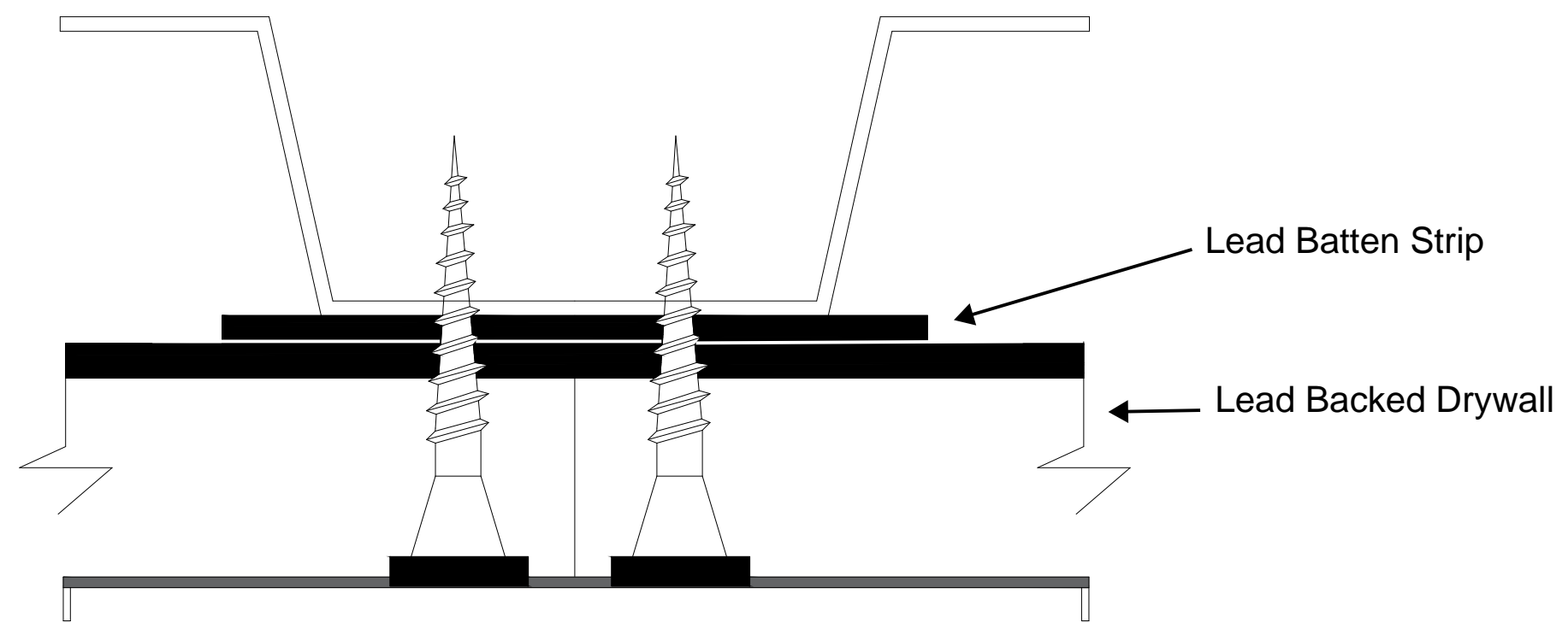
Lead batten strip at vertical joint Lead discs cover screw heads
