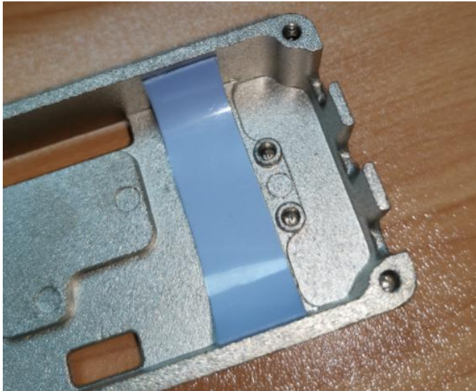
2.3、 Put MTVESC50A into upper cover and tightening A and B into mounting holes.
