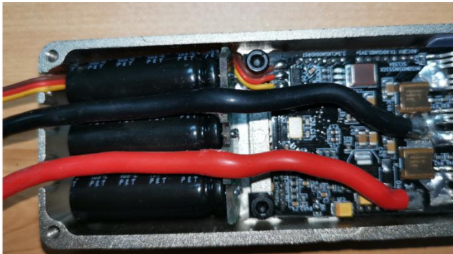
No heat-conducting silica tape between mosfets and bottom cover.
