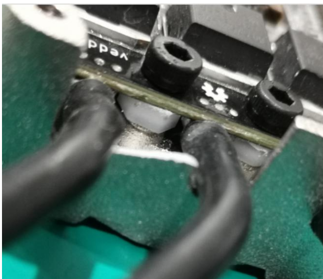
2.4、 Put the other piece of heat-conducting silica tape onto the other side MOSFETs.
