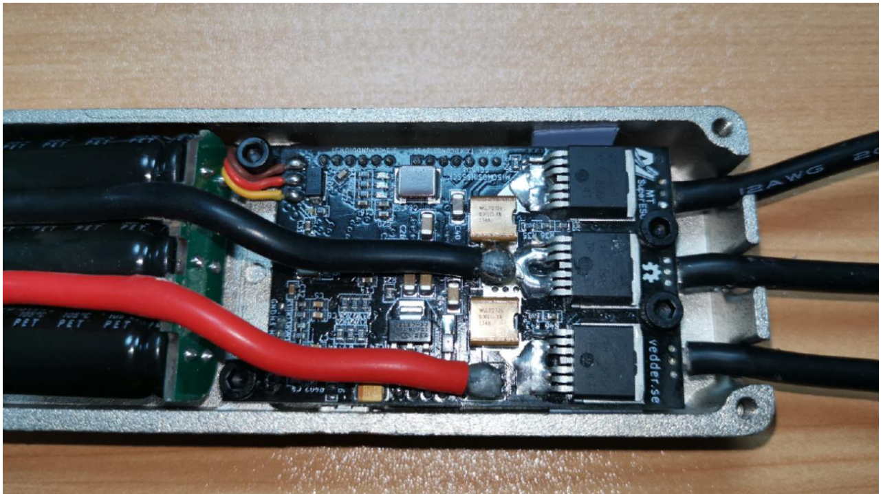
2.3、 Put MTVESC50A into upper cover and tightening A and B into mounting holes.
