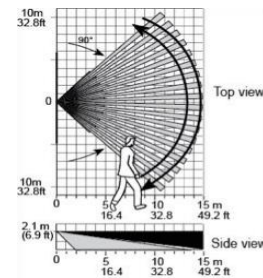
Figure 7 - Coverage Pattern Walk-Test
