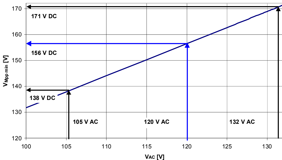
Fig. 4.1: Minimum MPP voltage as a function of grid voltage
