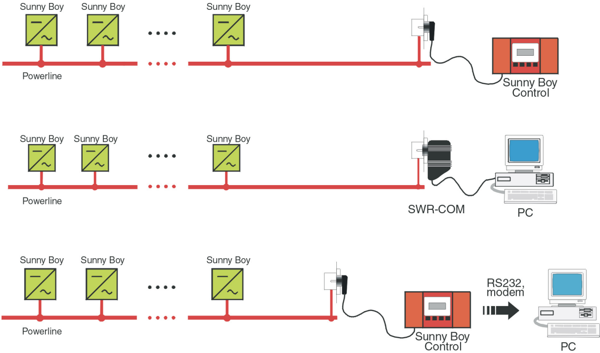
Fig. 3.1: Example of data transmission via Powerline
