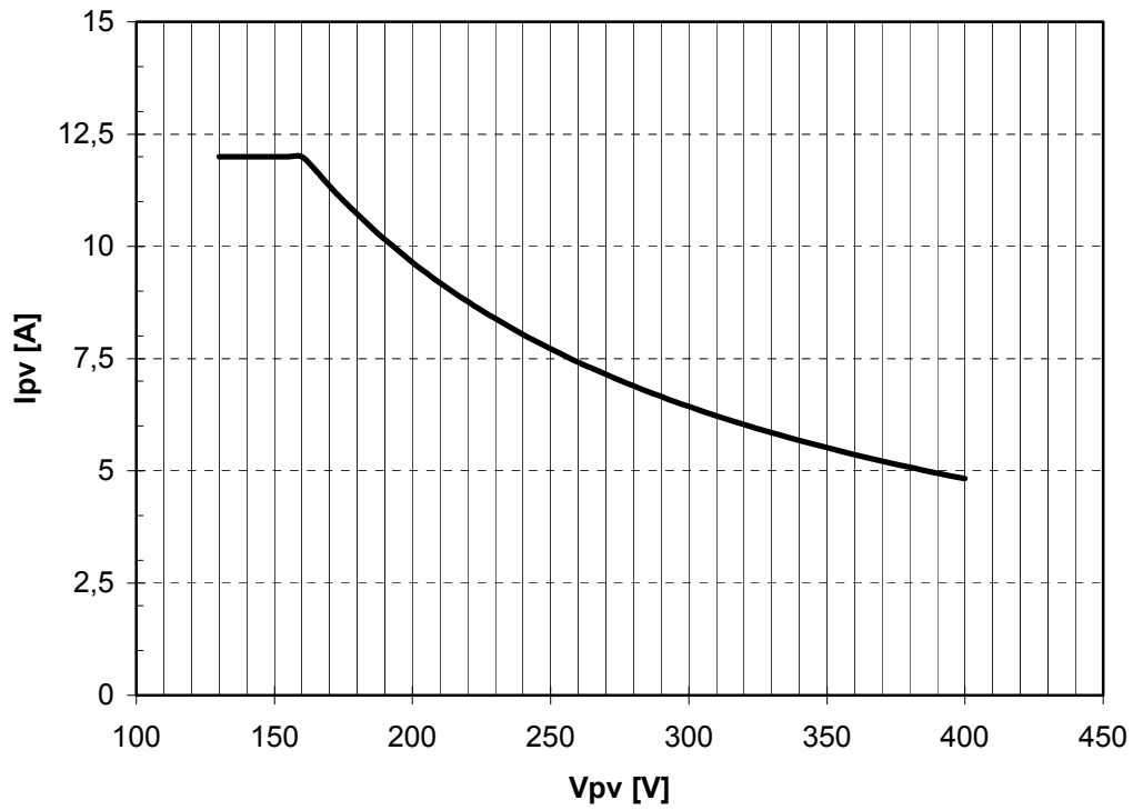
Fig. 4.2: Maximum Input Current of the Sunny Boy 1800U
