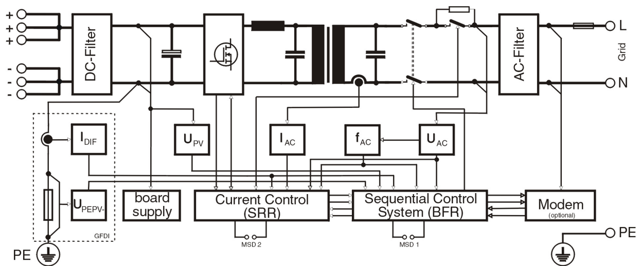
Fig. 2.2: Block circuit diagram of the Sunny Boy 1800U
