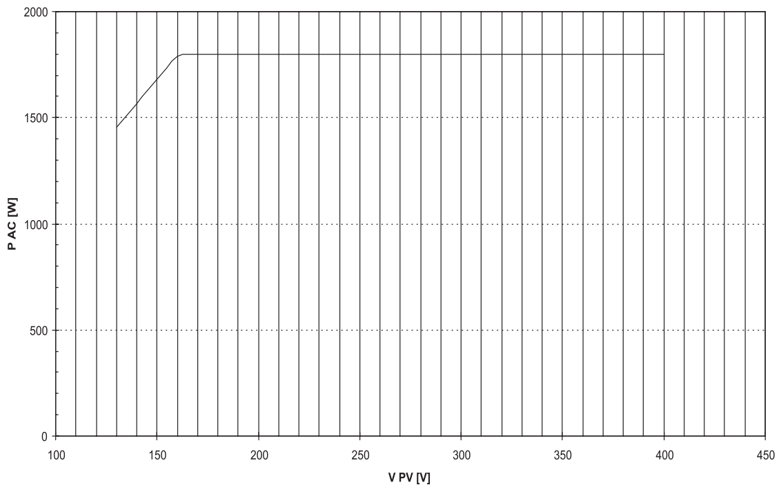
Fig. 4.3: Output Power of the Sunny Boy 1800U
