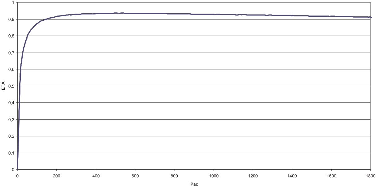
Fig. 4.4: Efficiency of the Sunny Boy 1800U
