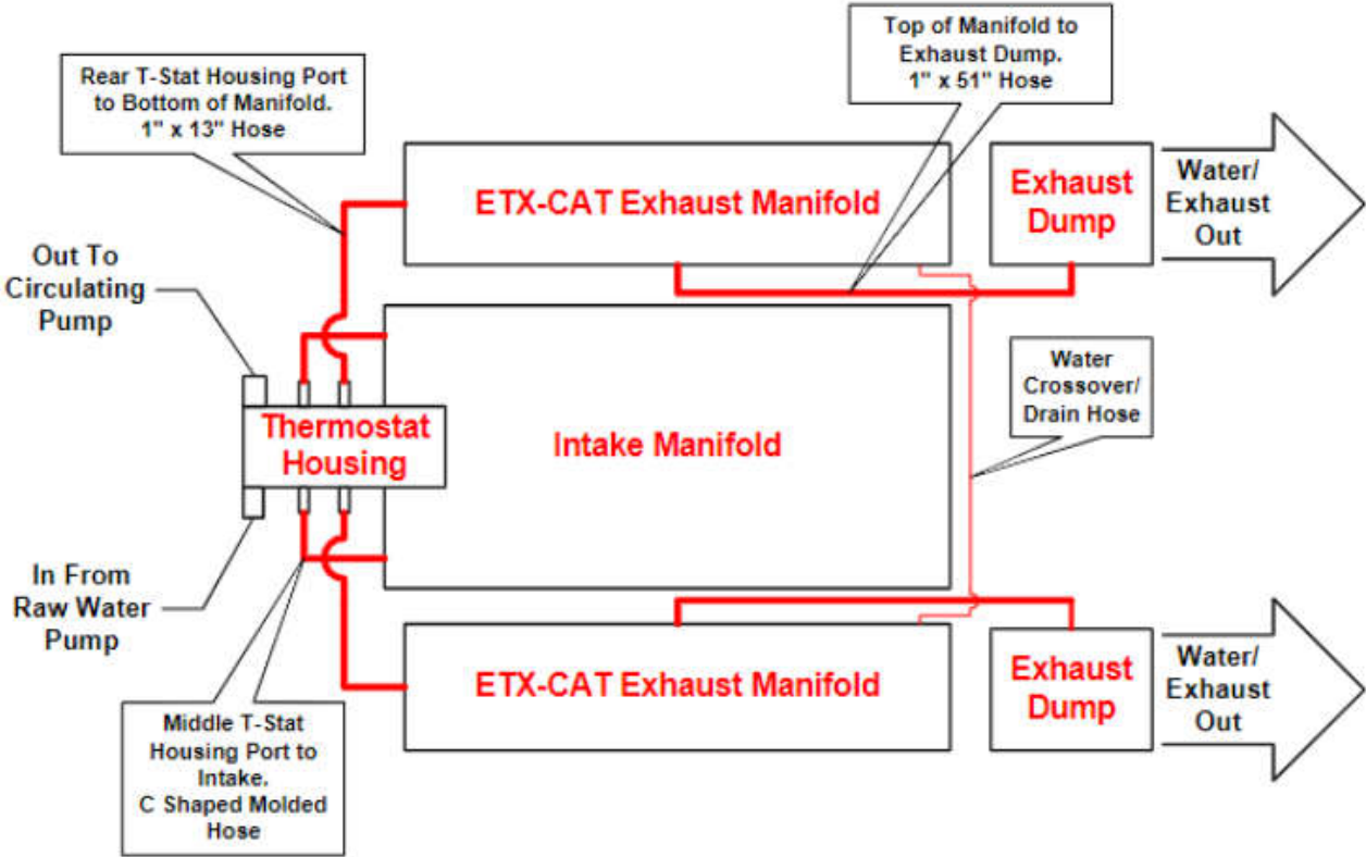
Replumb Flow Diagram
