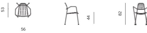
_ALU CHAIR DIMENSIONS 56x53x82 CM
