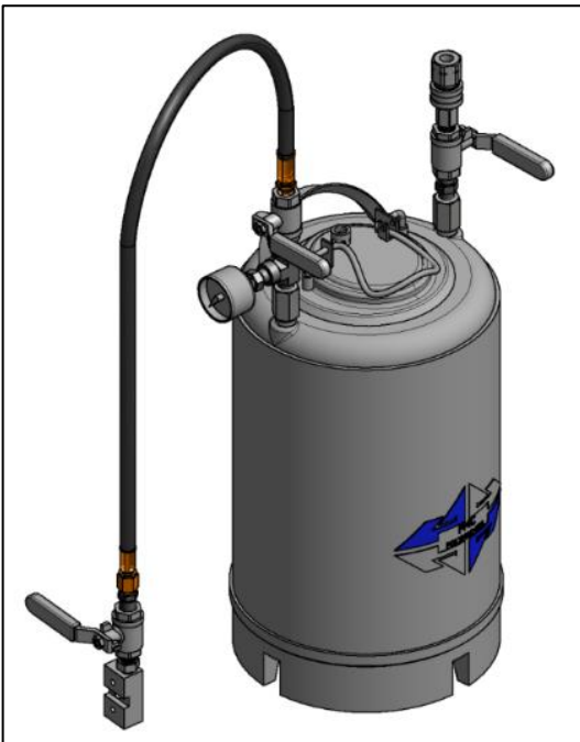
Figure 17: 2.5 Gallon Flush Tank (200426)
