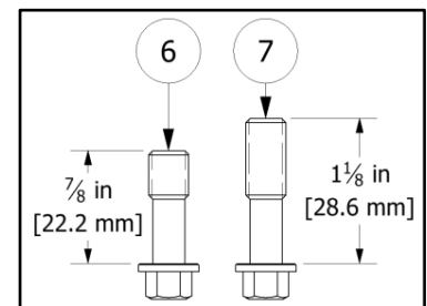
MOUNTING SCREWS
