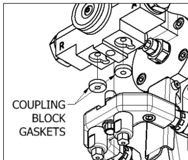
Figure 7: Coupling Block Gaskets
