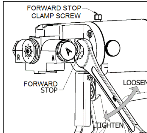
Figure 12: Valving Rod Adjustment
