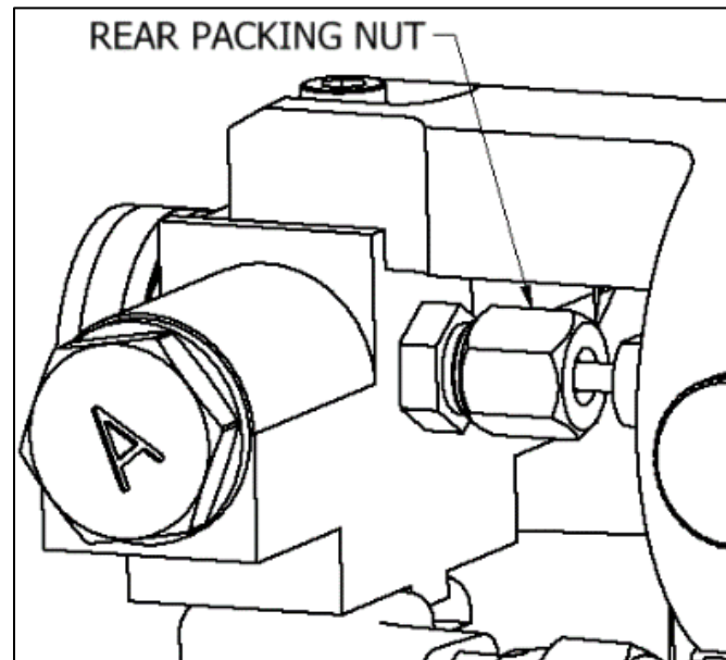
Figure 13: Rear Packing Nut
