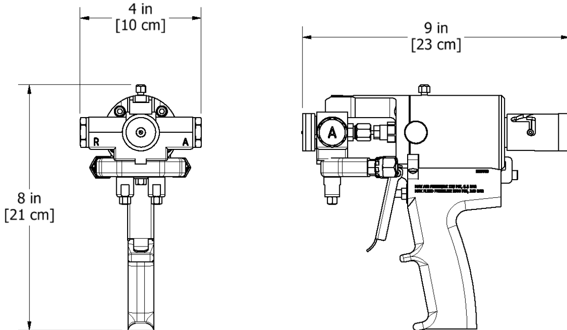
Figure 1: PX-7 Dimensions
