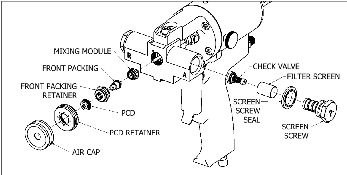
Figure 16: Clean Parts
