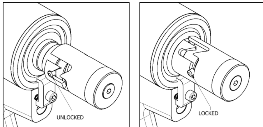
Figure 4: Safety Stop
