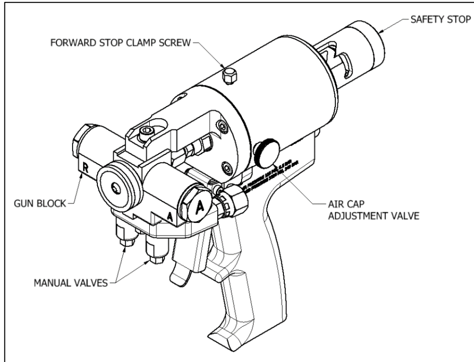
Figure 2: PX-7 Overview
