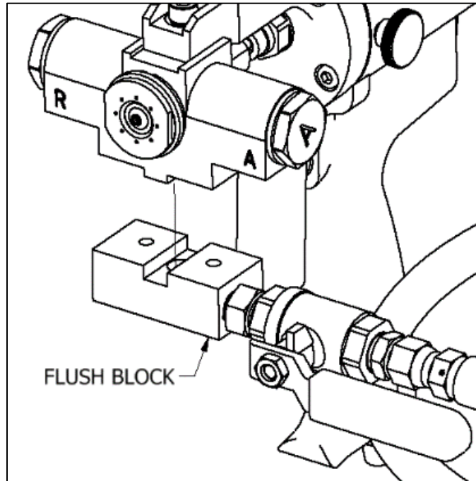
Figure 15: Flush Block Installation
