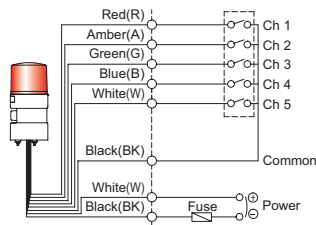
STND125R/STND125L/STND125LR-DC/AC
