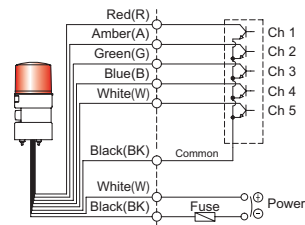
STND125DL-DC/AC
