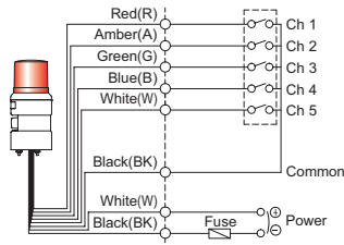
STND100R/STND100L/STND100LR-DC/AC
