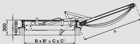
with PVC curb 16/00
