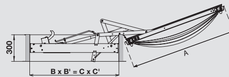
with metal curb M30
