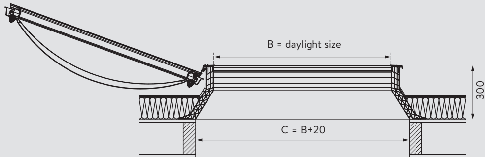
with PVC curb 30/20 (Installation in timber roof construction)
