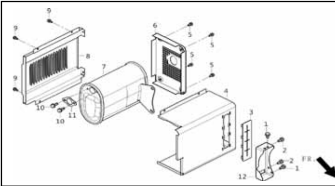
Fig. 13 - Muffler Assembly
