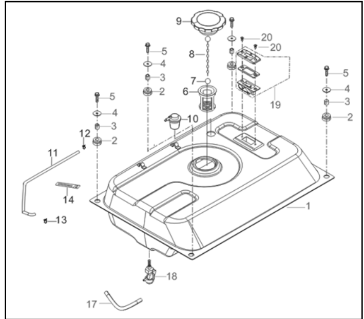
Fig. 14 - Tank, Fuel
