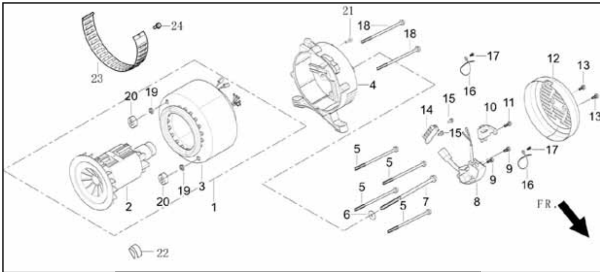
Fig. 18 - Rotor/Stator
