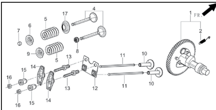
Fig. 6 - Valve/Camshaft Assembly
