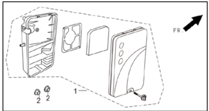
Fig. 10 - Air Cleaner
