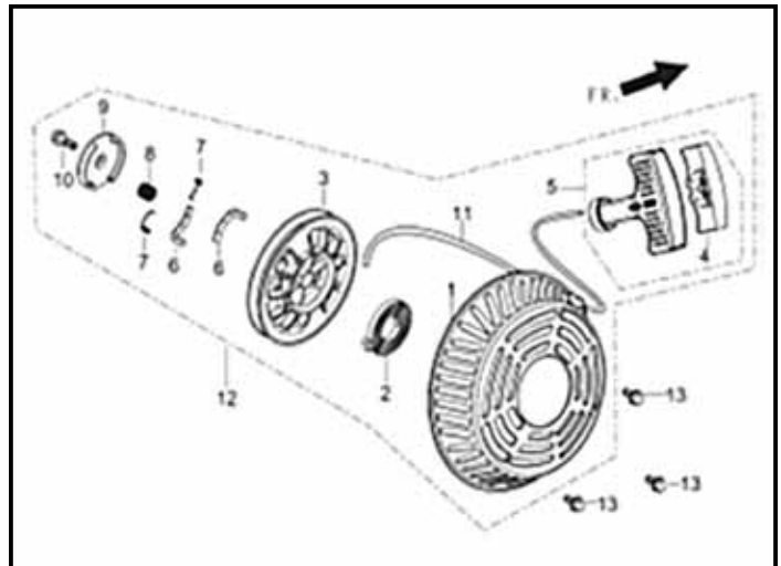
Fig. 7 - Recoil Starter
