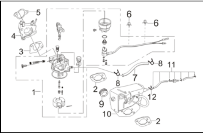
Fig. 9 - Carburetor Assembly
