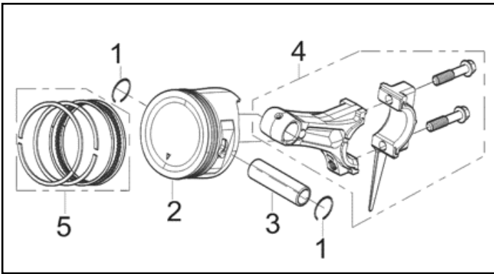
Fig. 5 - Piston Ring/Connecting Rod
