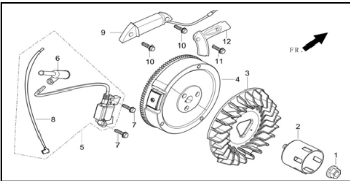
Fig. 11 - Flywheel/Ignition Coil
