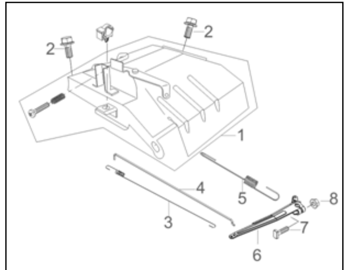
Fig. 12 - Control Assembly
