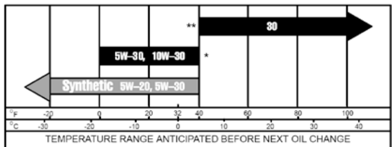
Fig. 1 - Engine Oil Temperature Recommendation
