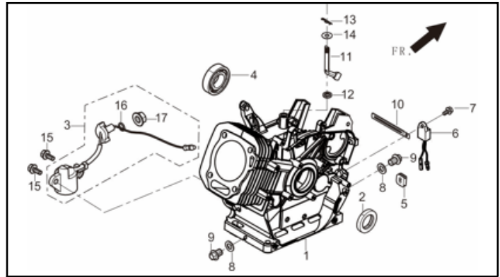
Fig. 2 - Crankcase Assembly
