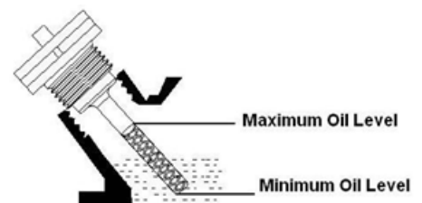
Fig. 10 - Oil Fill Opening, Dipstick and Oil Level
