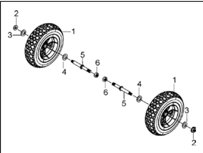
Fig. 15 - Wheel Assembly
