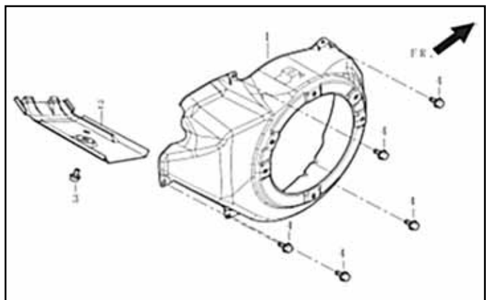
Fig. 8 - Shroud
