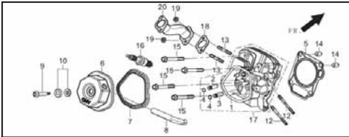
Fig. 1 - Cylinder Head Assembly
