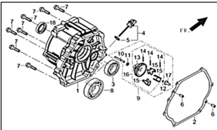
Fig. 3 - Crankcase Cover Assembly
