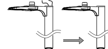
Connect wires inside mounting bracket
