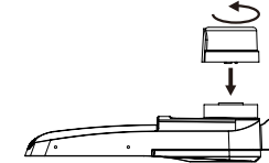
Install Photocell
