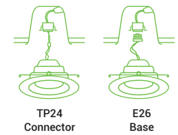
6" Housing
