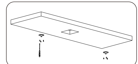
4. Screw the retaining disc to the wall
