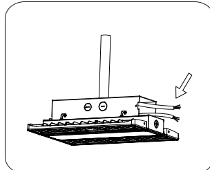
3. Wiring as required and taking safety precautions.
