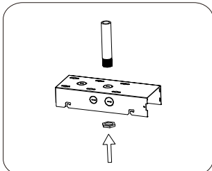
1. Install the junction box on the 3/4" pipe.
