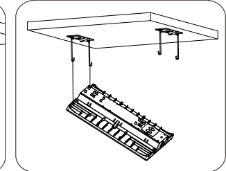
3. Insert hook ends into the holes of high bay light, as shown.
