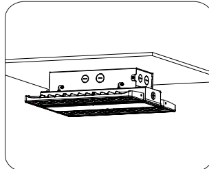
6. Complete installation.
