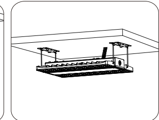
6. Insert hook ends into the holes of high bay light, as shown.
