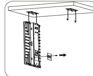
4. Remove the screws outside the wiring cover and remove the cover.
