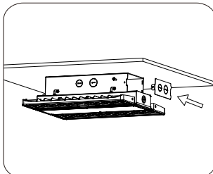
5. Close the cover and tighten the screws.
