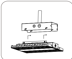
2. Install the light into the junction box and tighten the screws.
