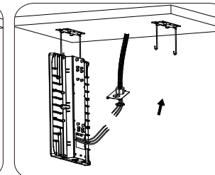
5. Pass the supply wires through the wiring cover and connect it with the fixture wire by color. Secure wiring cover by screws.
