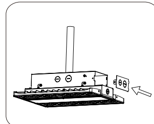
4. Close the cover and tighten the screws.
