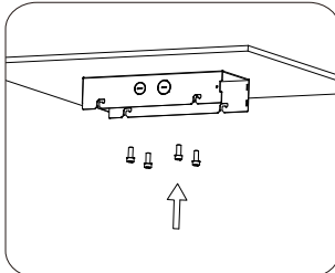
2. Mount the junction box to the ceiling.
