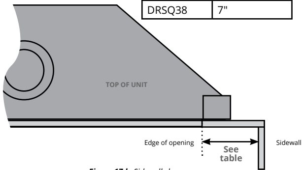
Figure 17.b Sidewall clearances
