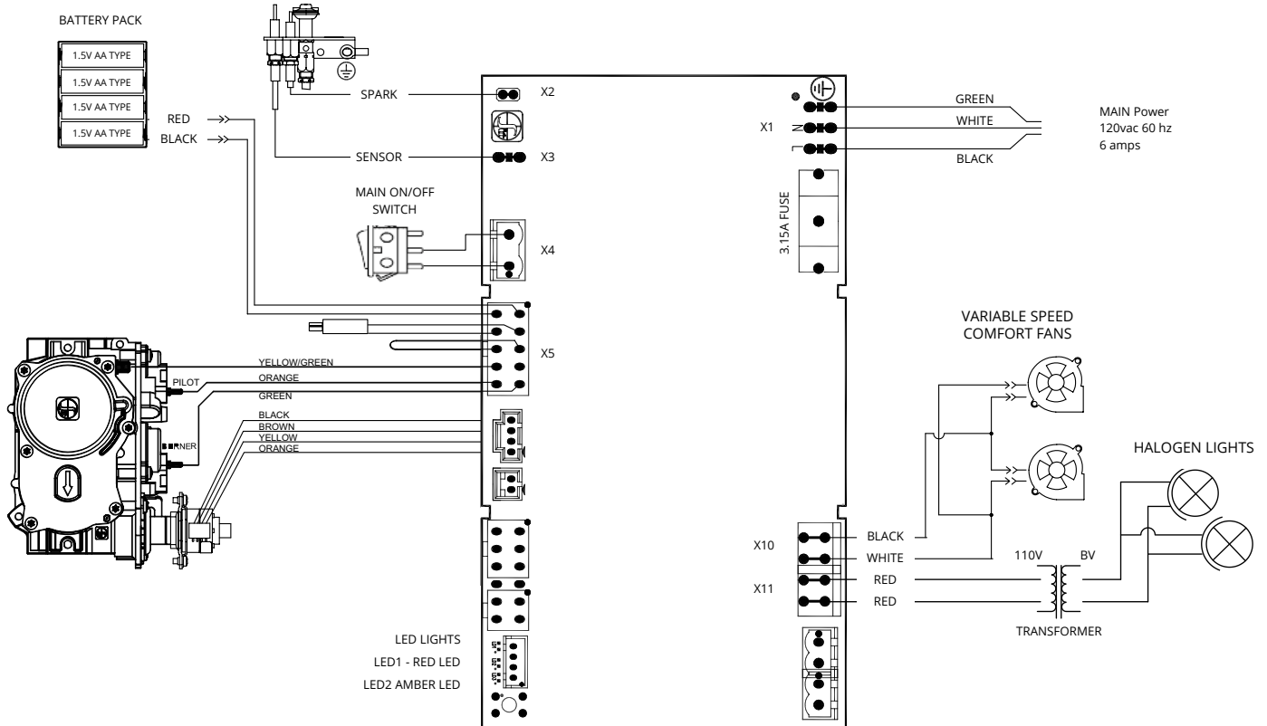
Figure 15b. Wiring diagram for DRSQ38*I-2 with SIT Prof flame Electronic Ignition
