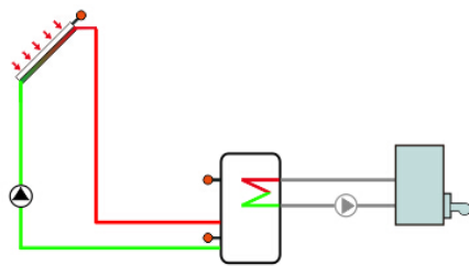
Back-up heating
