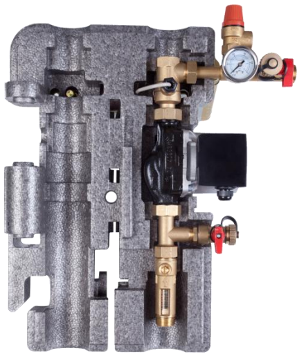
SR11series single pipe station
