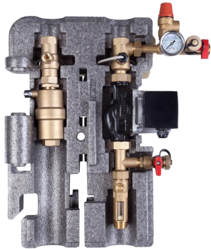
SR21series double pipes station
