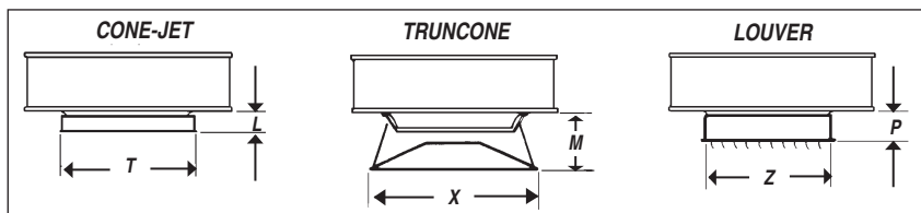
Figure 23.2 - Vertical Air Outlet Accessories
