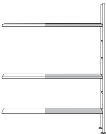
extension unit 01 1 side element, 3 shelves
