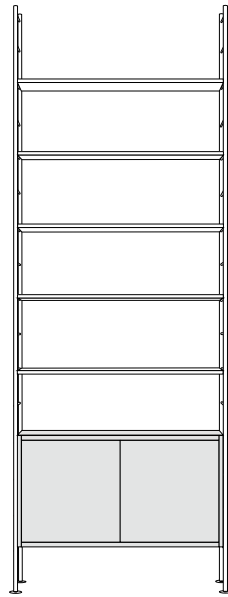
base unit 03 2 side elements, 5 shelves, 1 cabinet with 2 doors, wall brackets / set of 2
