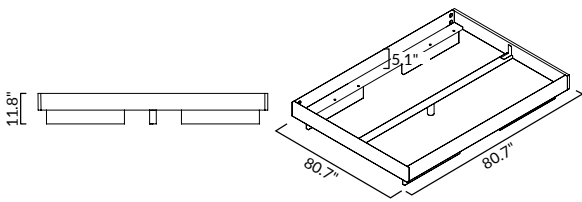
ZIANS Bed XLarge with continuous leg
