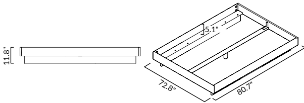
ZIANS Bed Large with continuous leg
