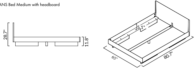
ZIANS Bed Medium with headboard and continuous leg
