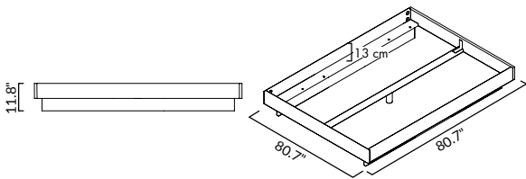
ZIANS Bed XLarge with continuous leg
