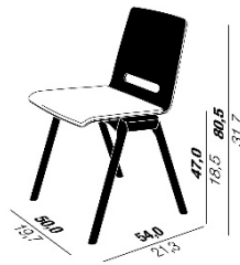
F2S-P0
