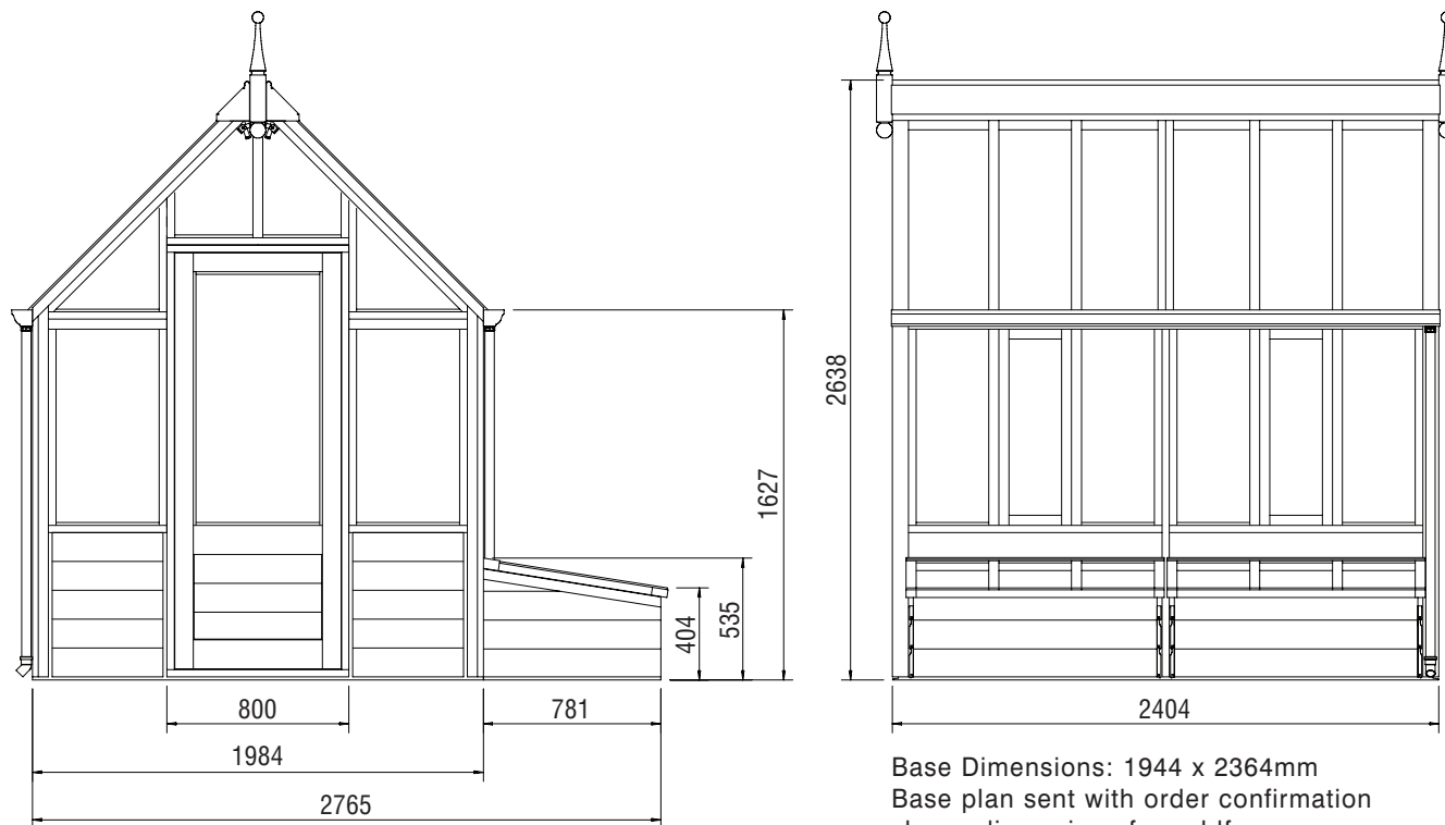
Approximate Greenhouse Dimensions: 6ft 6" x 8ft
